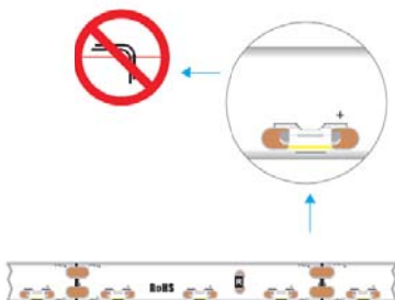
○ No bending the strip at the position of LED.
