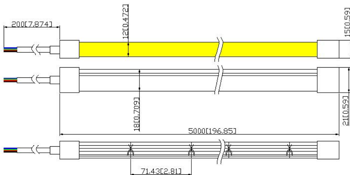
RX2284AP top outlet
