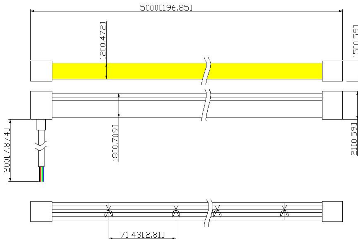
RX2284AP bottom outlet
