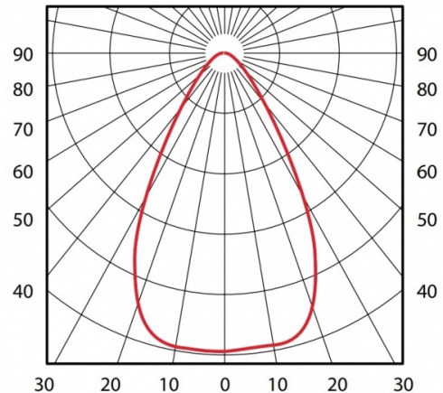
Mounting height 10-18 m
