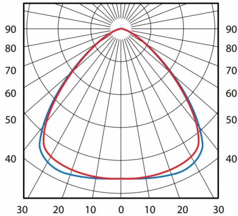
Mounting height 4-9 m
