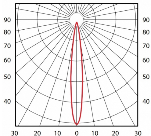
Mounting height 25-36 m
