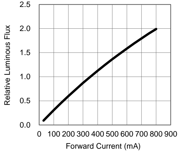
Fig 2. Relative Luminous Flux vs. Forward Current for White at T_j=25 maintained.
